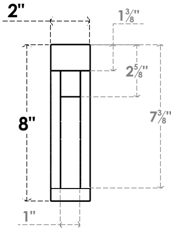
FRONT PROFILE
