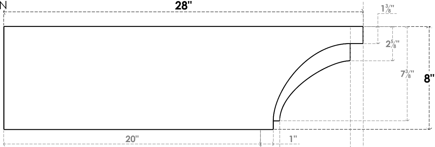
SIDE PROFILE
